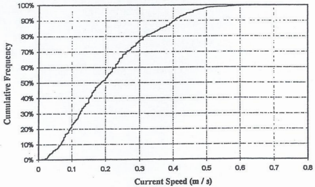
Cumulative Current Frequency at Peng Chau - Wet Season
