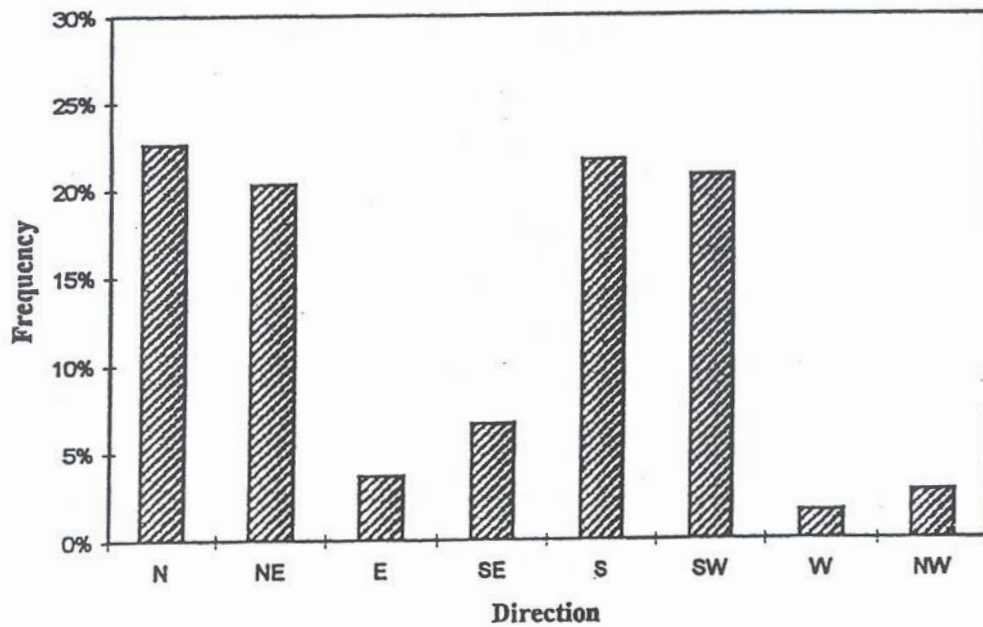
Distribution of Current Direction at Peng Chau - Wet Season
